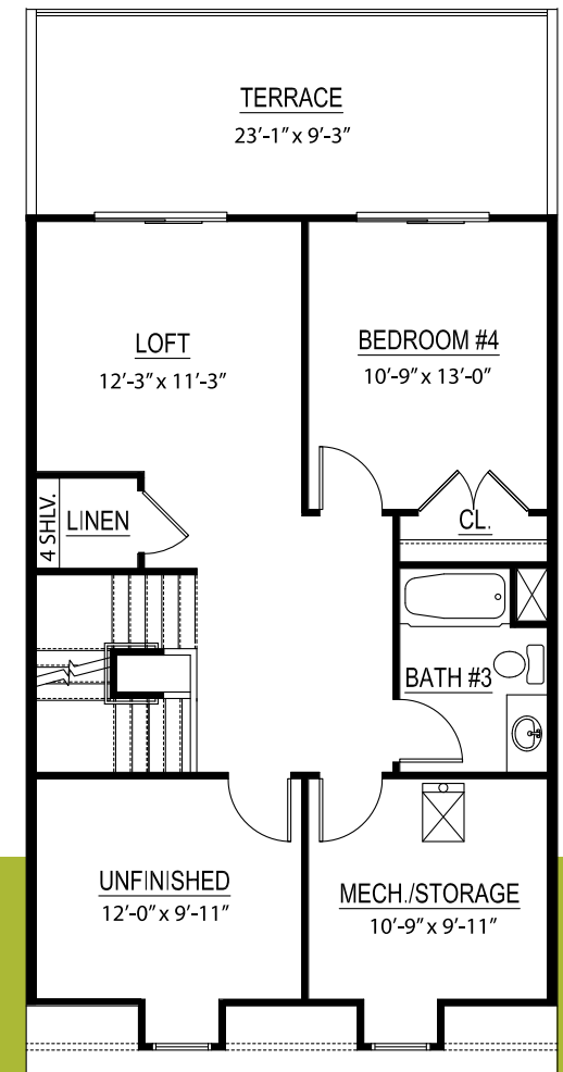
FOURTH FLOOR LOFT
