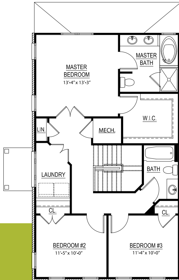
THIRD FLOOR
